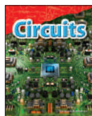
Circuits Grade 4 9781480746824 9781425846985
